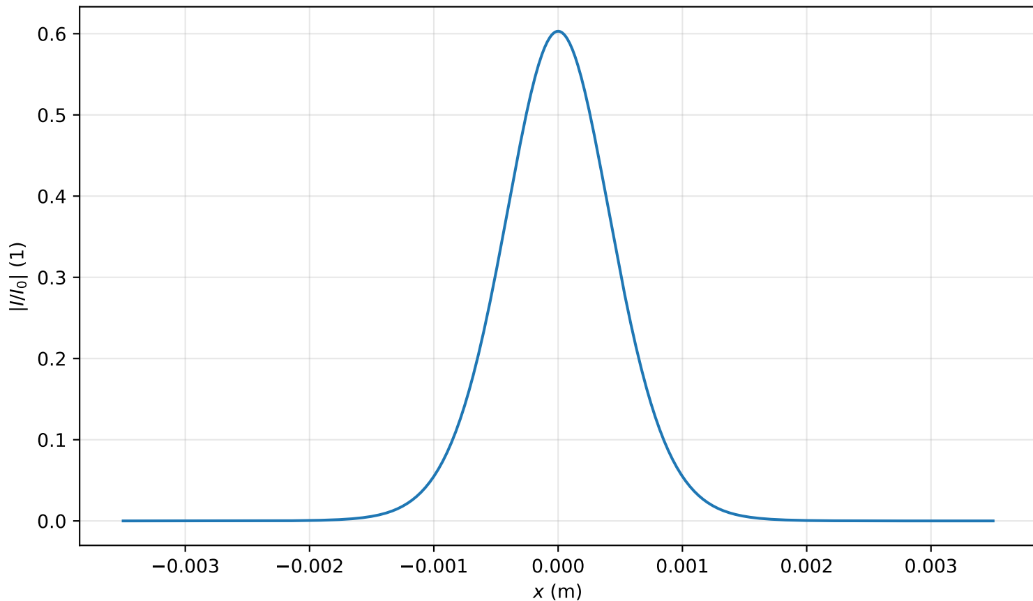
Intensity profile I(x, y = 0, z = 2.468m)/I_0 , P_{in}=0.4P_{cr} , artificial time
